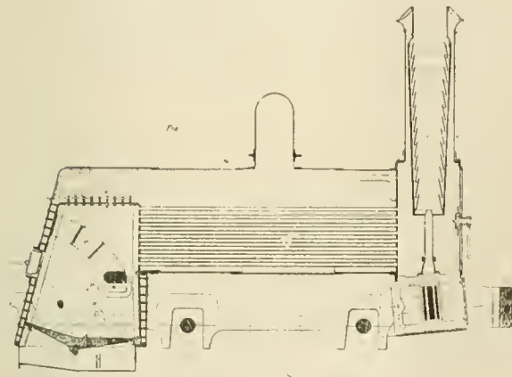
EATON'S SMOKE CONSUMING BOILER. FIG. 66.
